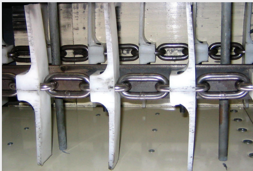
Bolt 'N' Go System Round Link Chain Application on a Conveyor
